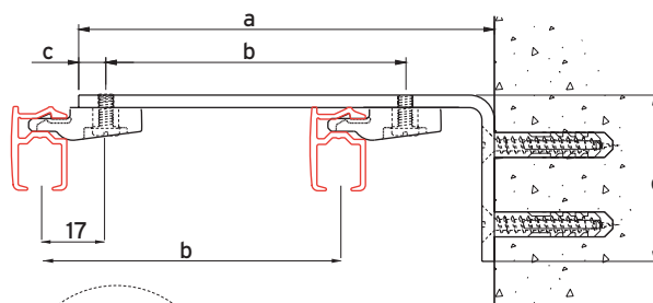
end view detail of extension bracket
