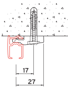
Top fixing with ceiling bracket 5350
