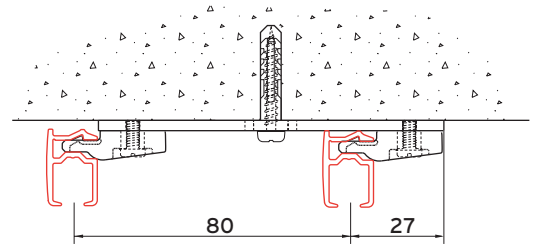
Top fixing with double bracket 2216-53 and ceiling bracket 5350
