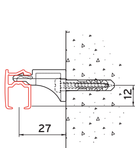
Face fixing with wall bracket 5351
